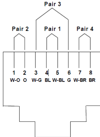
Figure 4: Eight-position jack pin/pair assignment (T568B)
