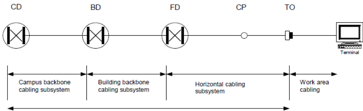
Fig.1 Generic Cabling system
