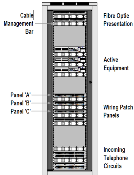
Figure 5: Cabinet Layout
