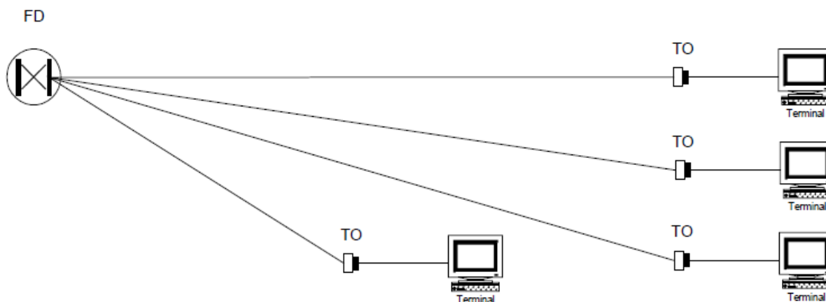
Fig. 3: Horizontal Cabling
