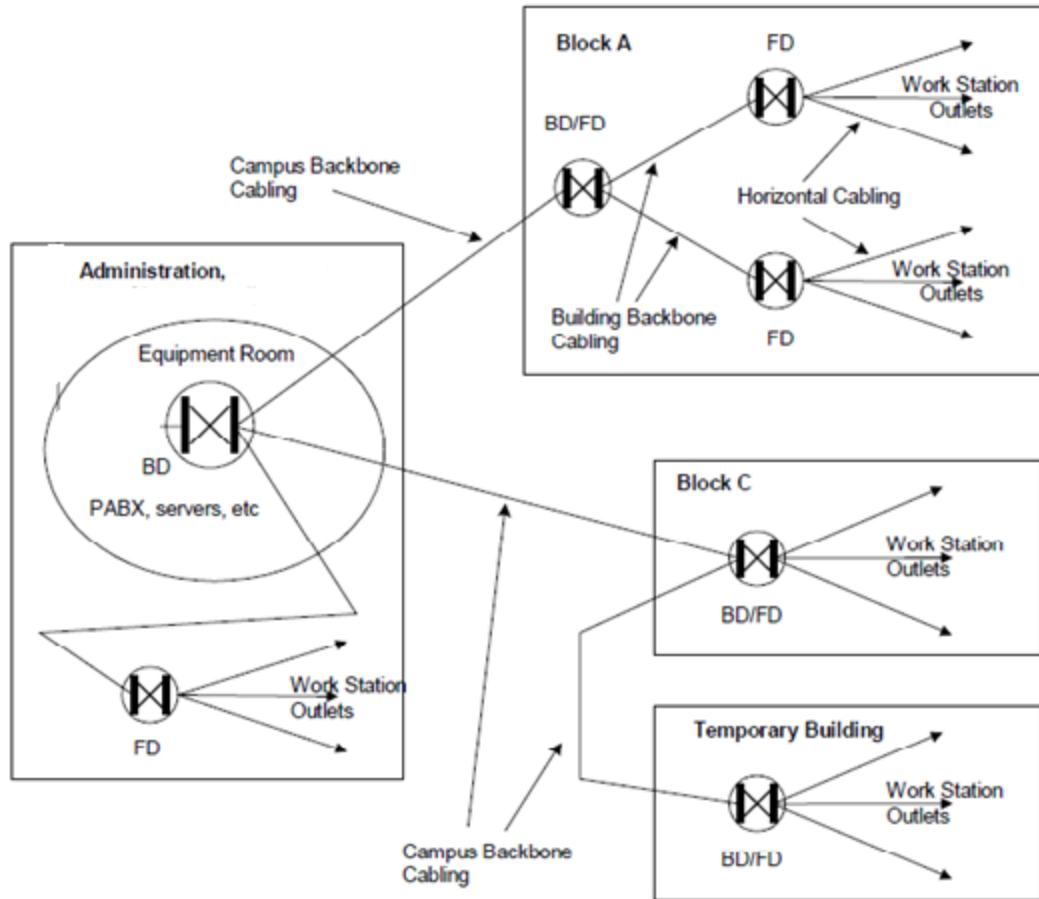
Fig. 2: Conceptual layout
